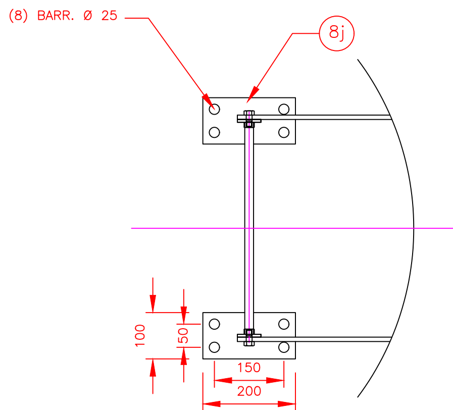
VISTA "E-E"
