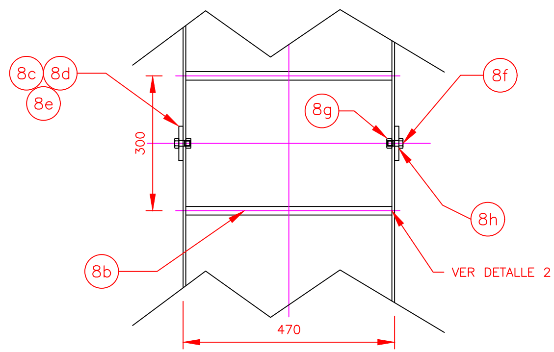
VISTA "D-D"
